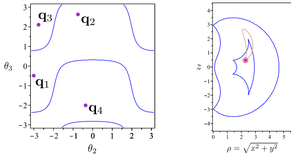
(a) Singularities in joint space (b) Singularities in workspace
