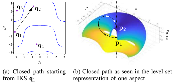
Fig. 7: An example of nonsingular change of solutions
