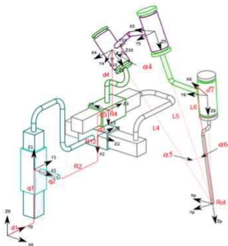
(a) Serial architecture of the Robotol
